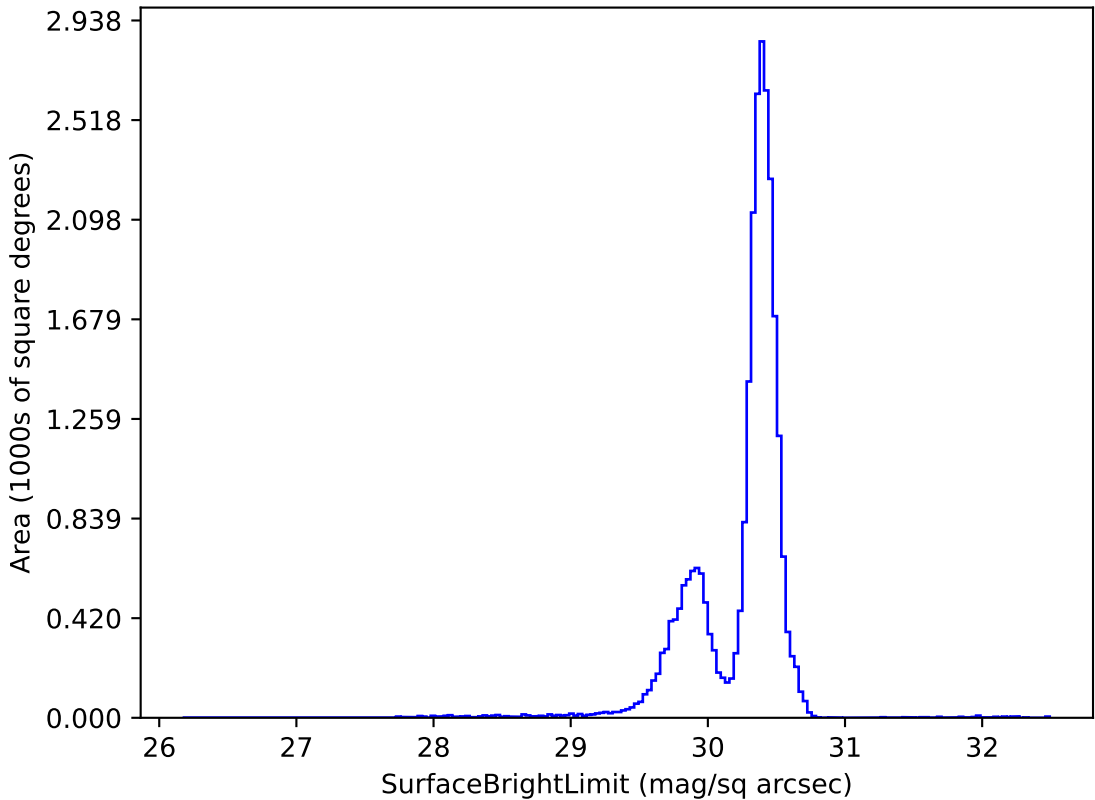
rolling_phased_ps_-182_psf_0_v3.3_10yrs g: SurfaceBrightLimit
