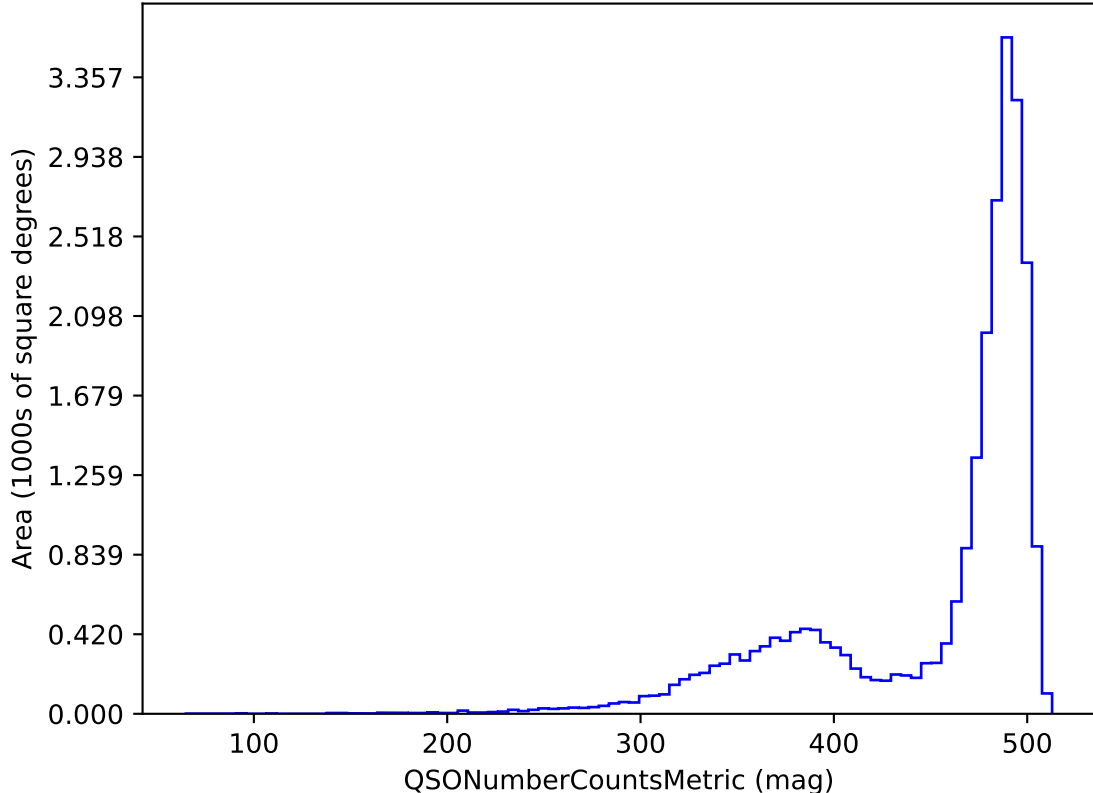
rolling_phased_ps_-182_psf_0_v3.3_10yrs z band and non-DD: QSONumberCountsMetric
