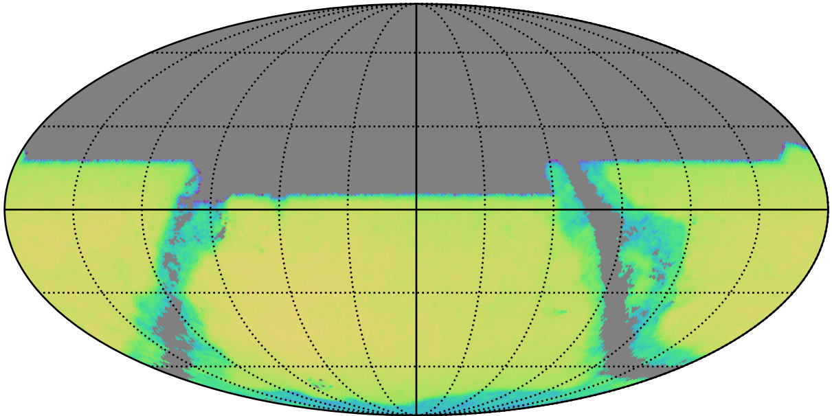
rolling_phased_ps_-182_psf_0_v3.3_10yrs y band and non-DD: QSONumberCountsMetric
