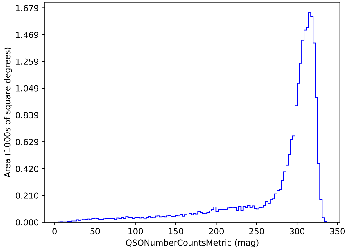
rolling_phased_ps_-182_psf_0_v3.3_10yrs u band and non-DD: QSONumberCountsMetric
