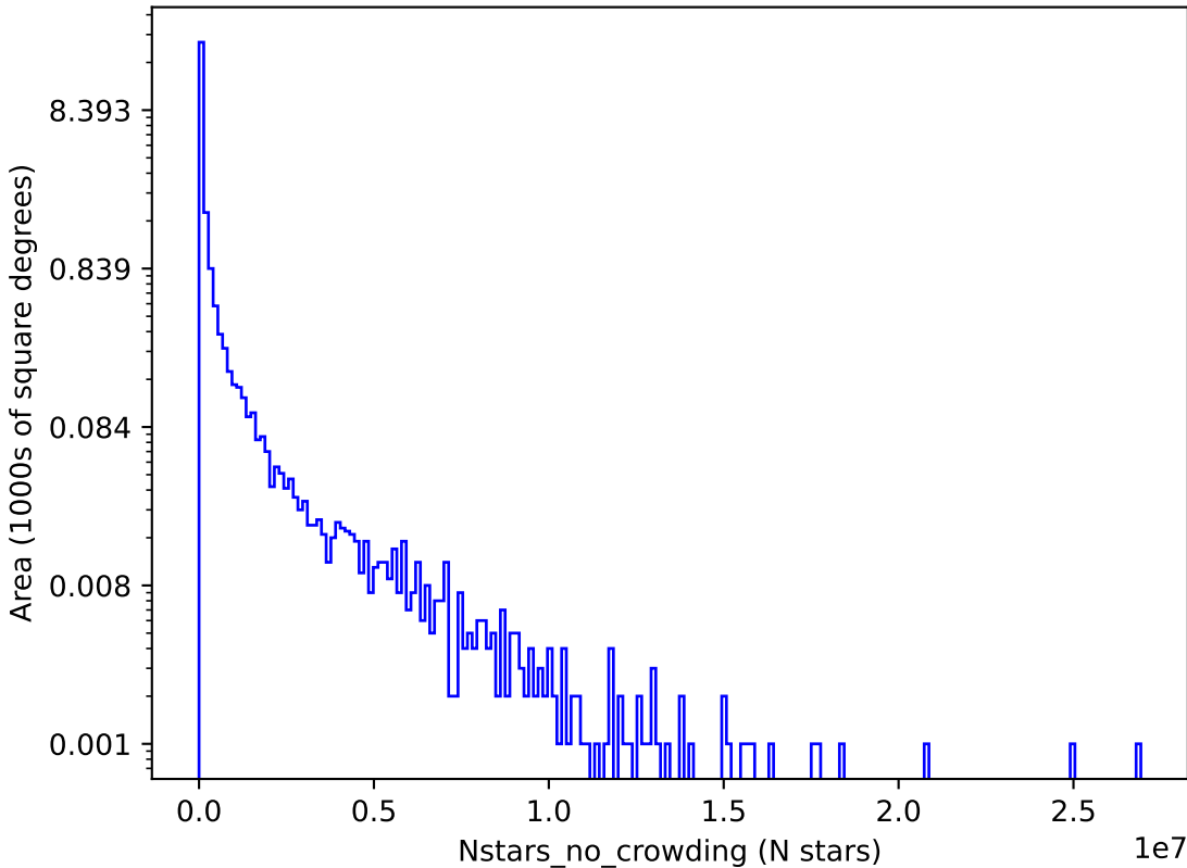
rolling_phased_ps_-182_psf_0_v3.3_10yrs z: Nstars_no_crowding
