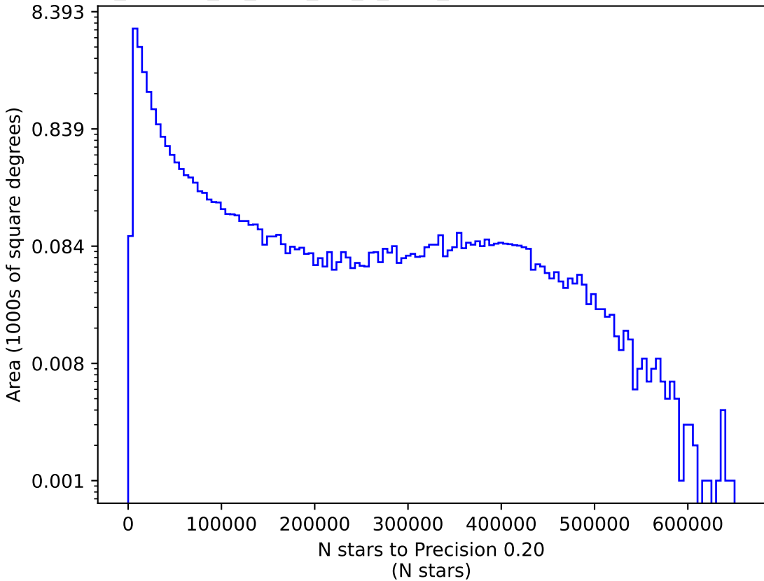
rolling_phased_ps_-182_psf_0_v3.3_10yrs z: N stars to Precision 0.20
