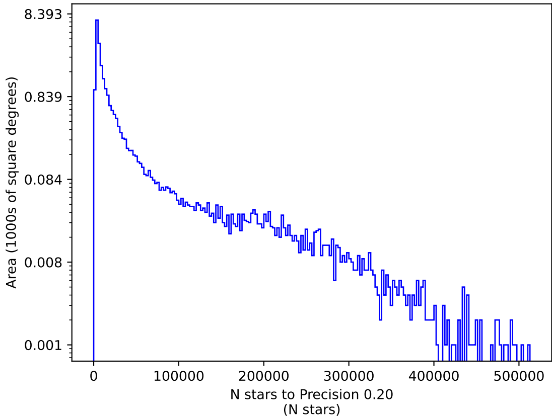
rolling_phased_ps_-182_psf_0_v3.3_10yrs u: N stars to Precision 0.20
