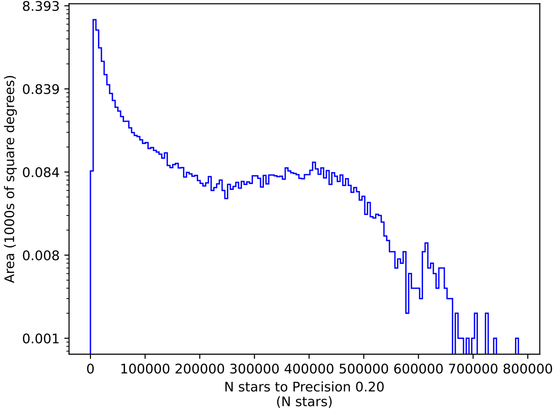
rolling_phased_ps_-182_psf_0_v3.3_10yrs i: N stars to Precision 0.20
