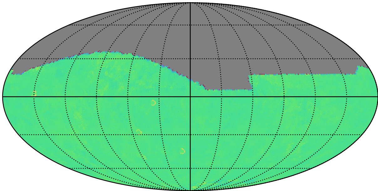
rolling_phased_ps_-182_psf_0_v3.3_10yrs z: Kuiper rotTelPos
