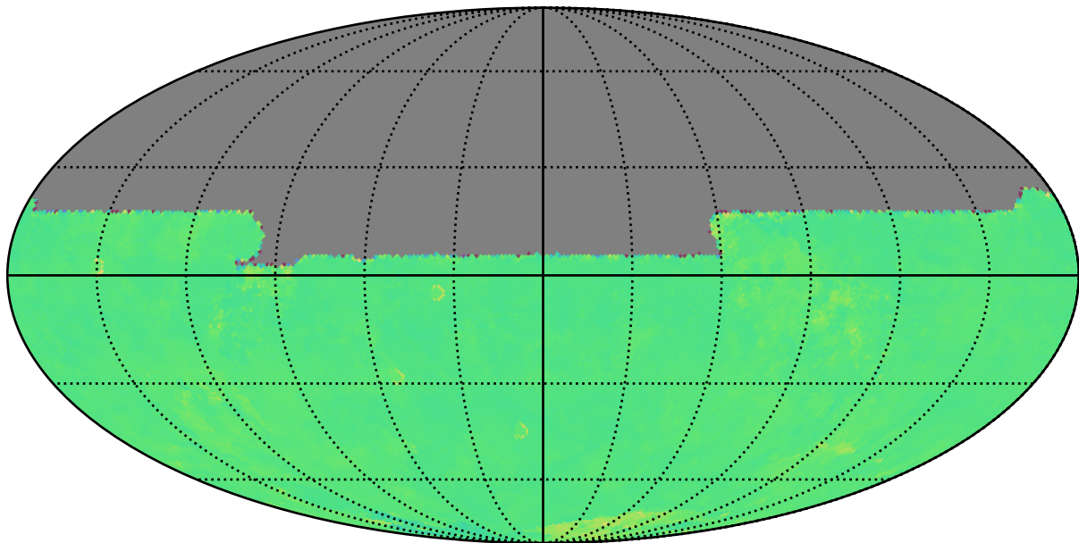
rolling_phased_ps_-182_psf_0_v3.3_10yrs y: Kuiper rotTelPos
