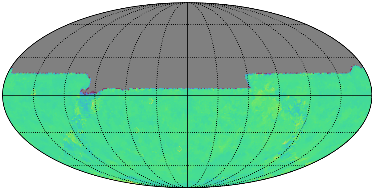
rolling_phased_ps_-182_psf_0_v3.3_10yrs u: Kuiper rotTelPos
