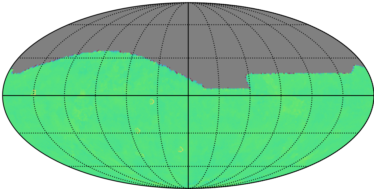
rolling_phased_ps_-182_psf_0_v3.3_10yrs i: Kuiper rotTelPos
