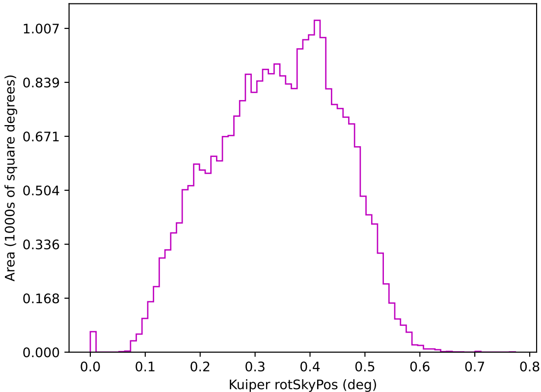
rolling_phased_ps_-182_psf_0_v3.3_10yrs z: Kuiper rotSkyPos
