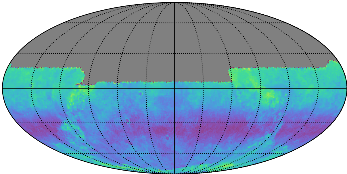
rolling_phased_ps_-182_psf_0_v3.3_10yrs y: Kuiper rotSkyPos
