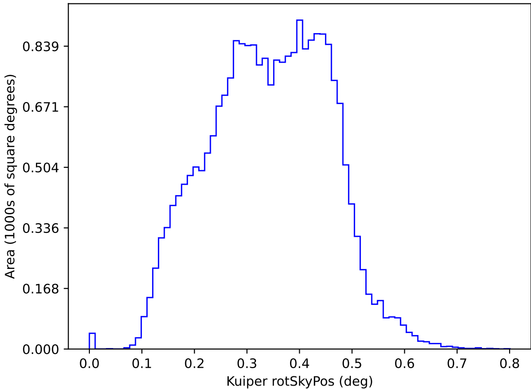
rolling_phased_ps_-182_psf_0_v3.3_10yrs y: Kuiper rotSkyPos
