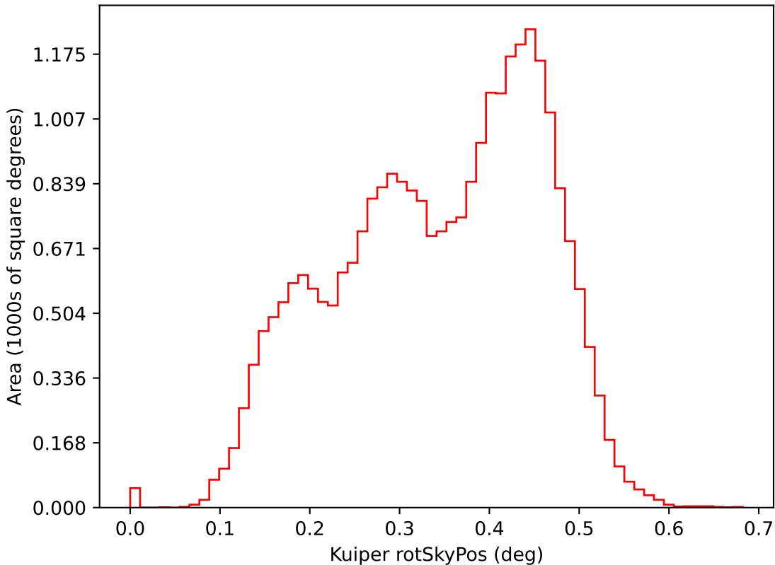
rolling_phased_ps_-182_psf_0_v3.3_10yrs i: Kuiper rotSkyPos
