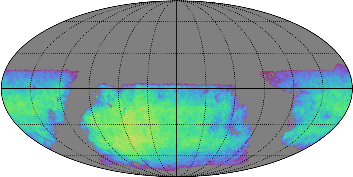
rolling_phased_ps_-182_psf_0_v3.3_10yrs i band non-DD year 8: ExgalM5WithCuts
