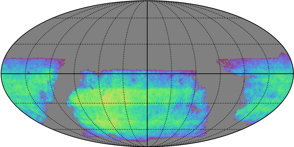
rolling_phased_ps_-182_psf_0_v3.3_10yrs i band non-DD year 6: ExgalM5WithCuts
