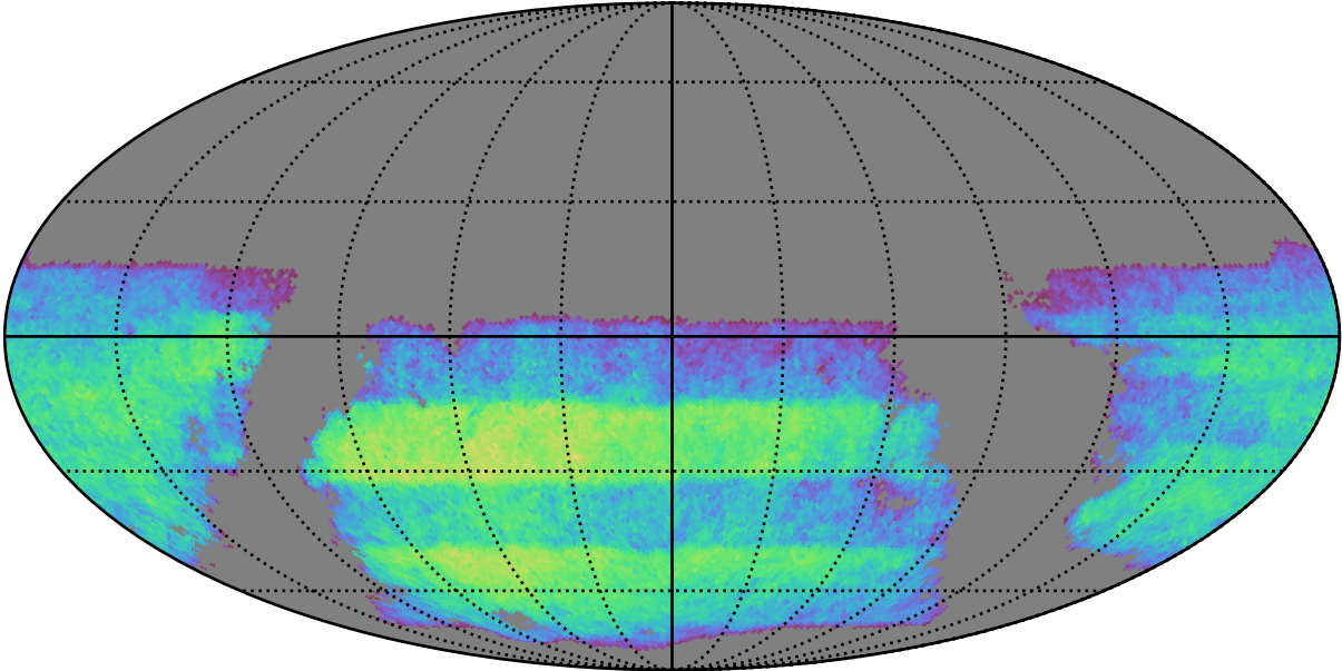
rolling_phased_ps_-182_psf_0_v3.3_10yrs i band non-DD year 3: ExgalM5WithCuts
