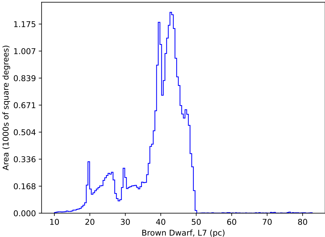
rolling_phased_ps_-182_psf_0_v3.3_10yrs : Brown Dwarf, L7
