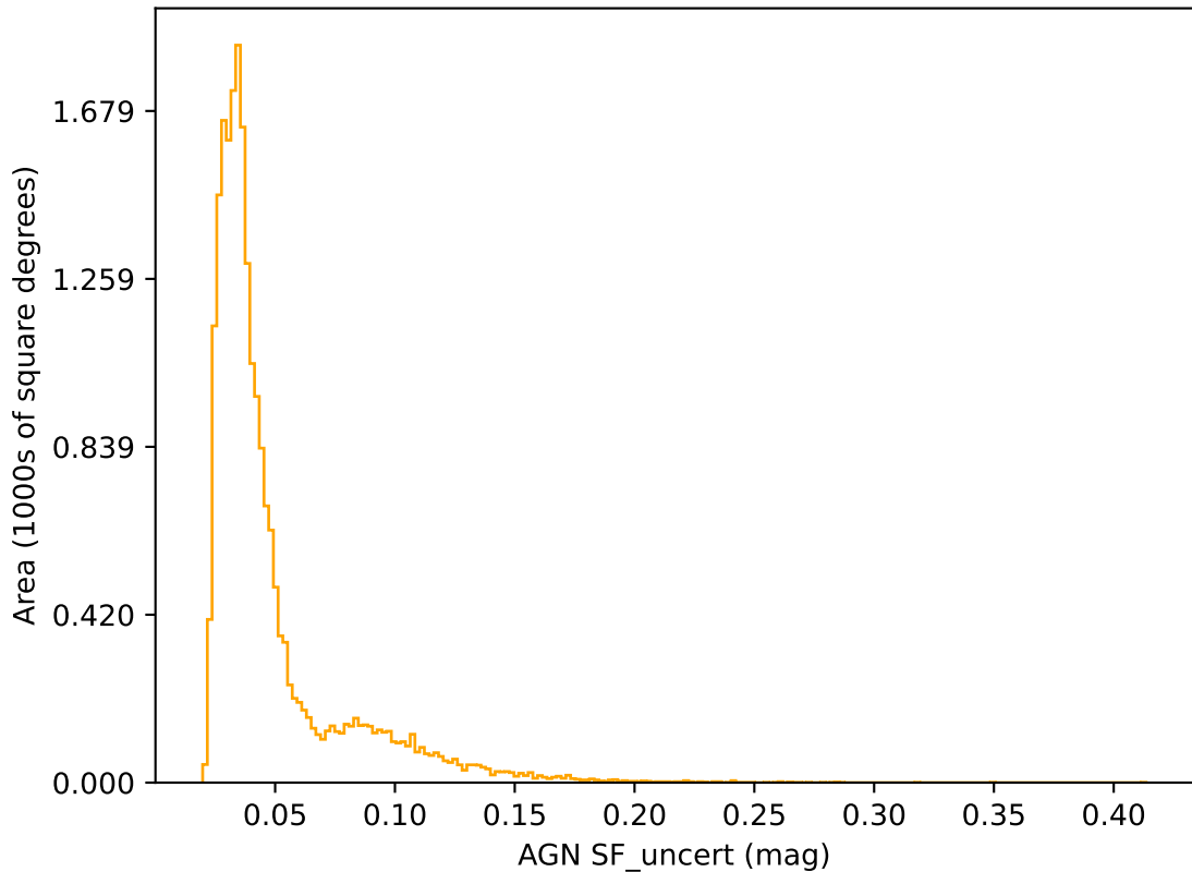
rolling_phased_ps_-182_psf_0_v3.3_10yrs r band: AGN SF_uncert
