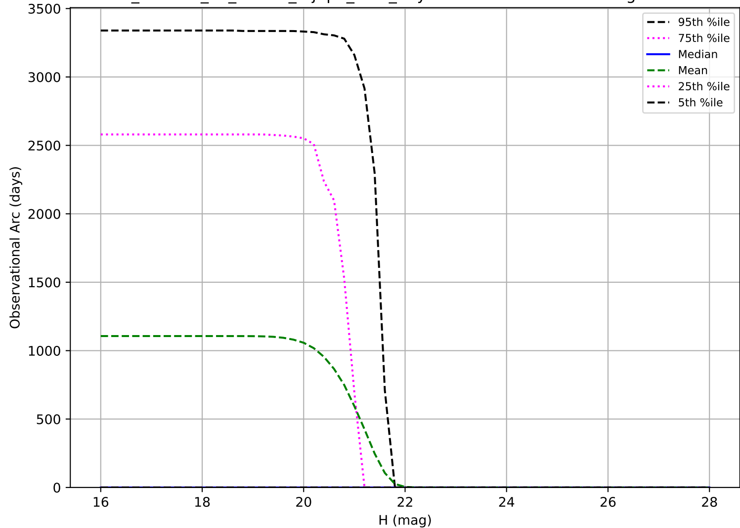
roll_uniform_eh_acc1.0_mjdp0_v3.4_10yrs: Observational Arc Length Vatira
