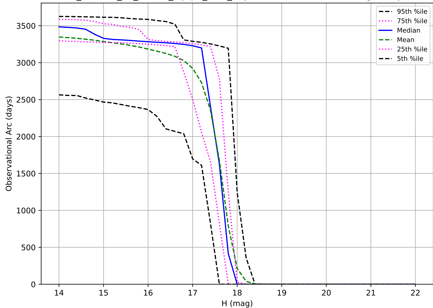
roll_uniform_eh_acc1.0_mjdp0_v3.4_10yrs: Observational Arc Length Trojan
