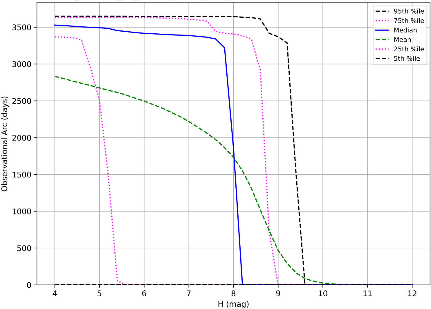
roll_uniform_eh_acc1.0_mjdp0_v3.4_10yrs: Observational Arc Length TNO
