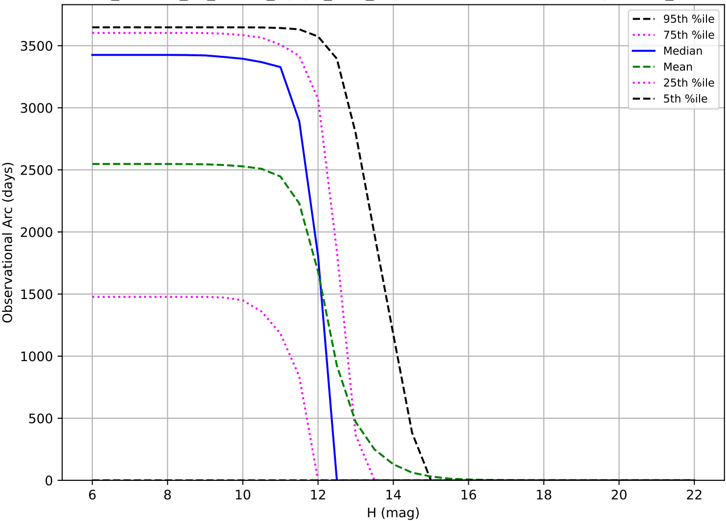
roll_uniform_eh_acc1.0_mjdp0_v3.4_10yrs: Observational Arc Length OCC_r20
