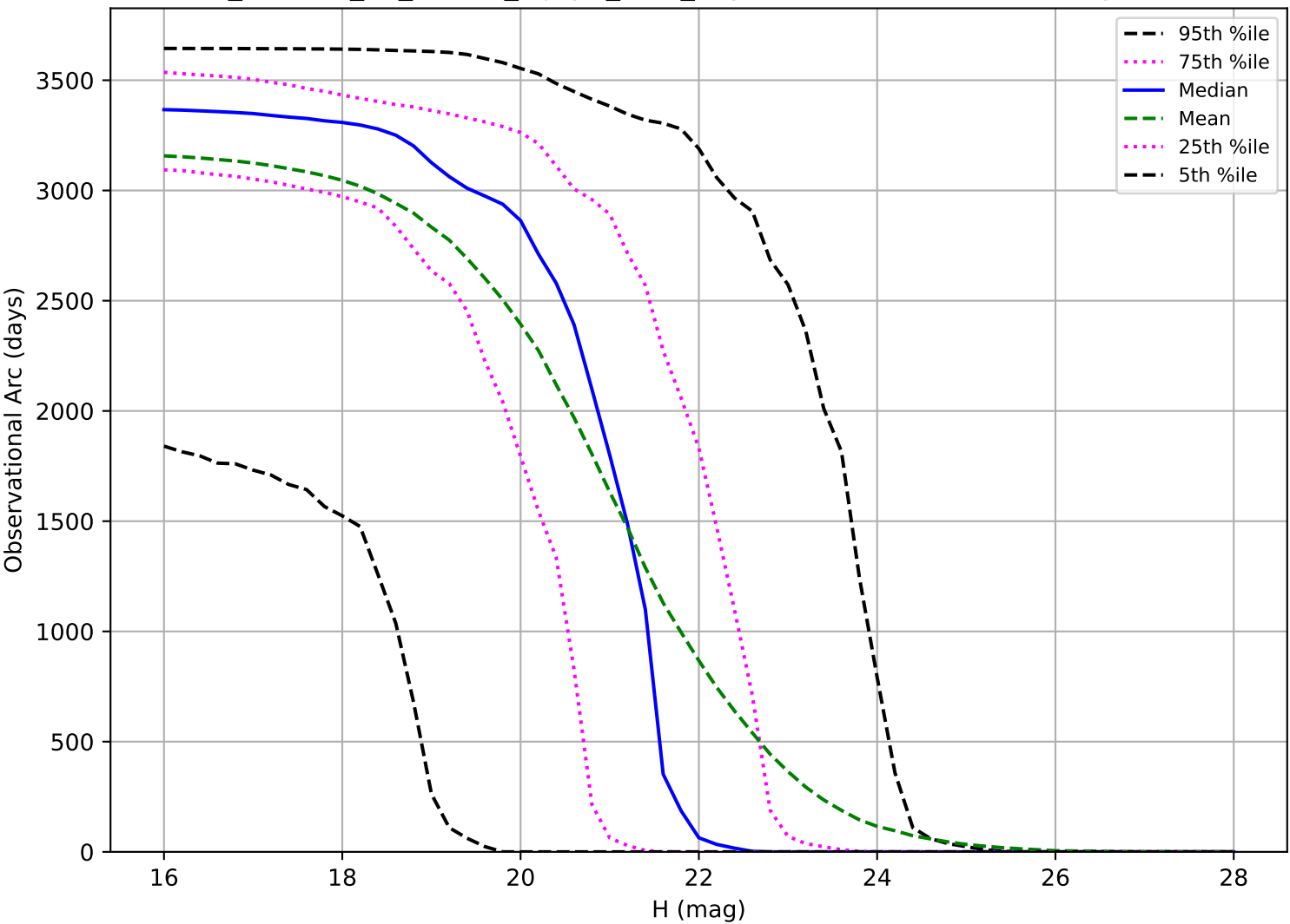
roll_uniform_eh_acc1.0_mjdp0_v3.4_10yrs: Observational Arc Length NEO
