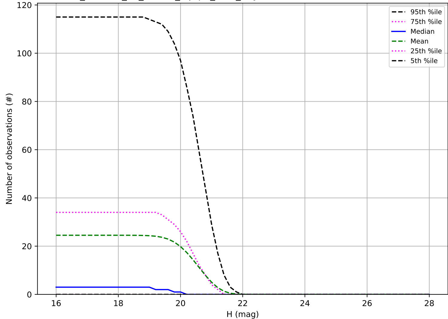
roll_uniform_eh_acc1.0_mjdp0_v3.4_10yrs: Number of observations Vatira
