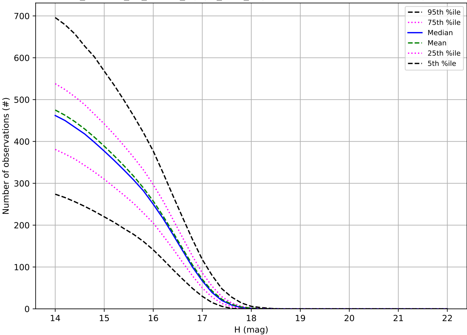
roll_uniform_eh_acc1.0_mjdp0_v3.4_10yrs: Number of observations Trojan
