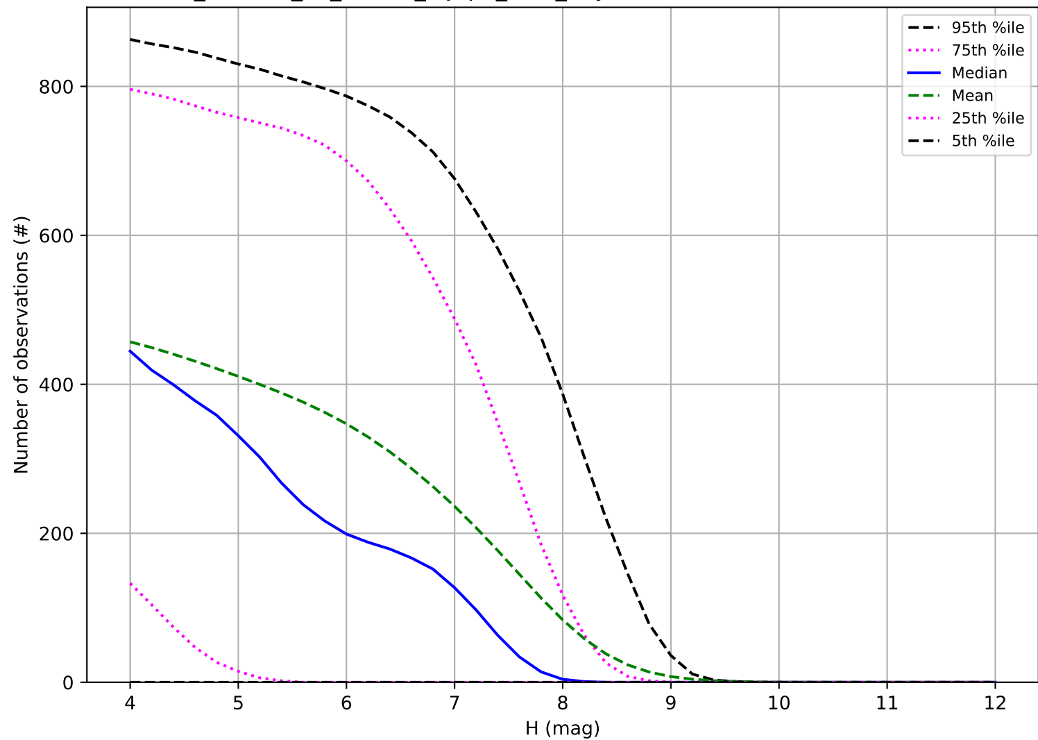
roll_uniform_eh_acc1.0_mjdp0_v3.4_10yrs: Number of observations TNO
