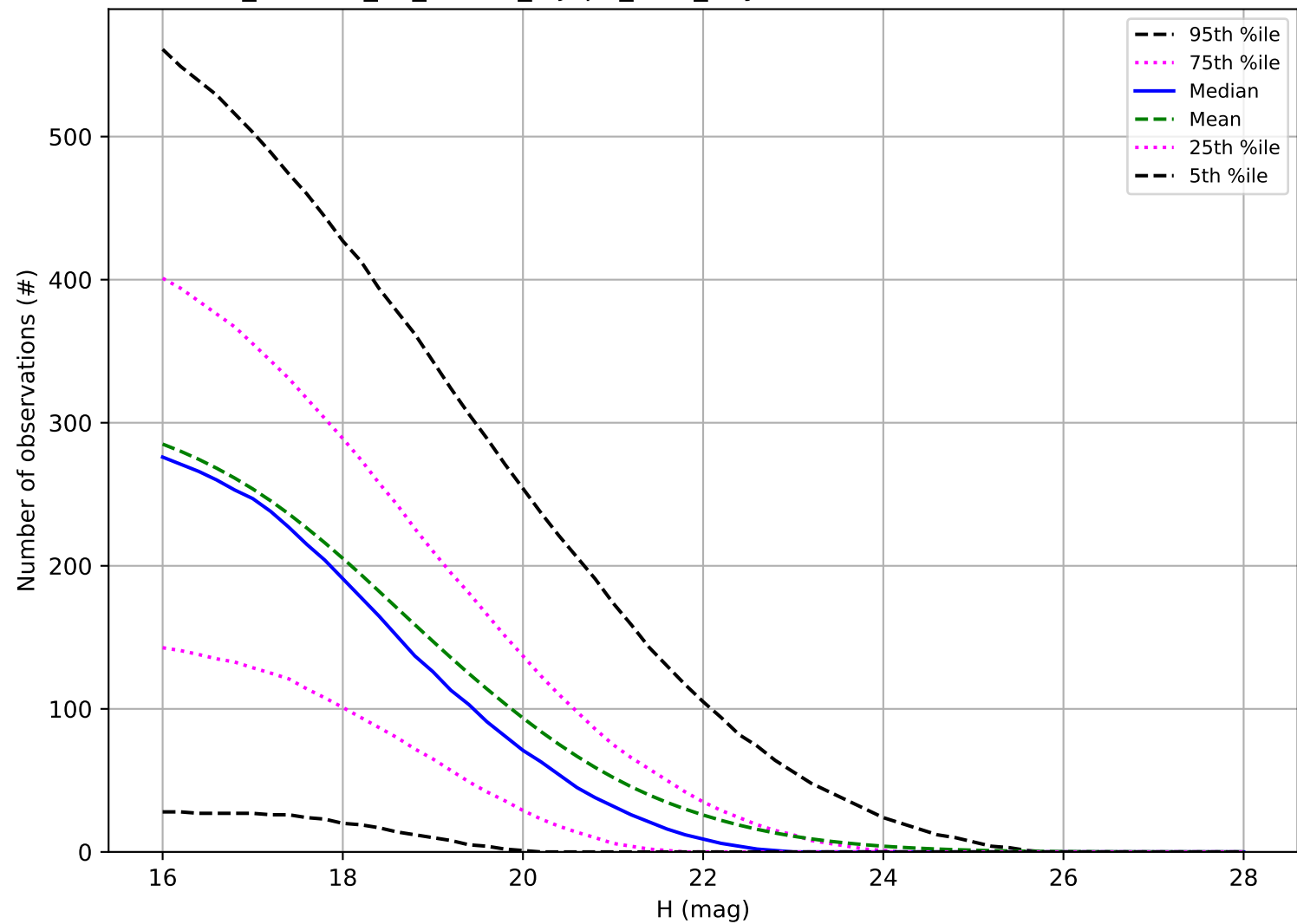
roll_uniform_eh_acc1.0_mjdp0_v3.4_10yrs: Number of observations NEO
