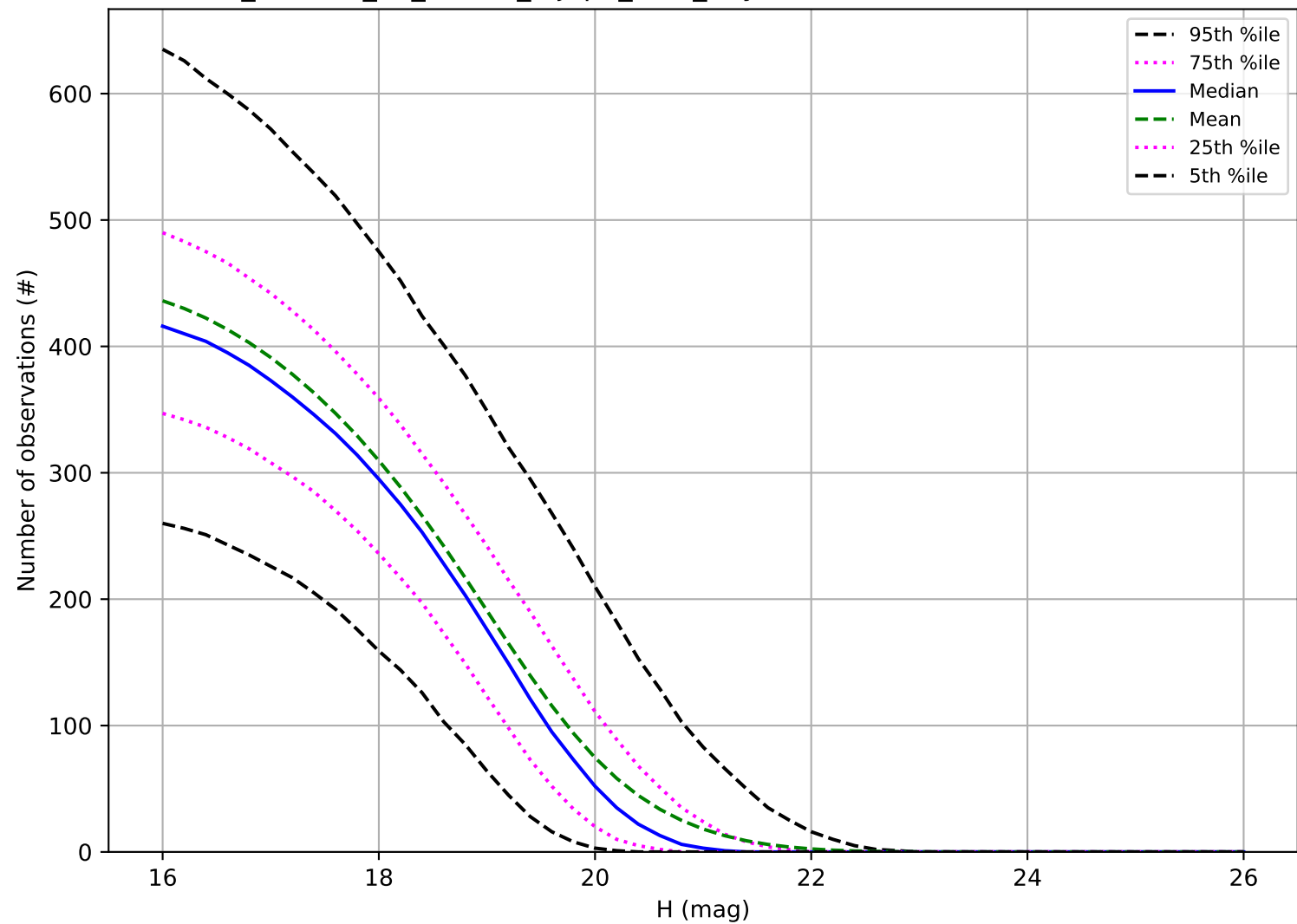
roll_uniform_eh_acc1.0_mjdp0_v3.4_10yrs: Number of observations MBA
