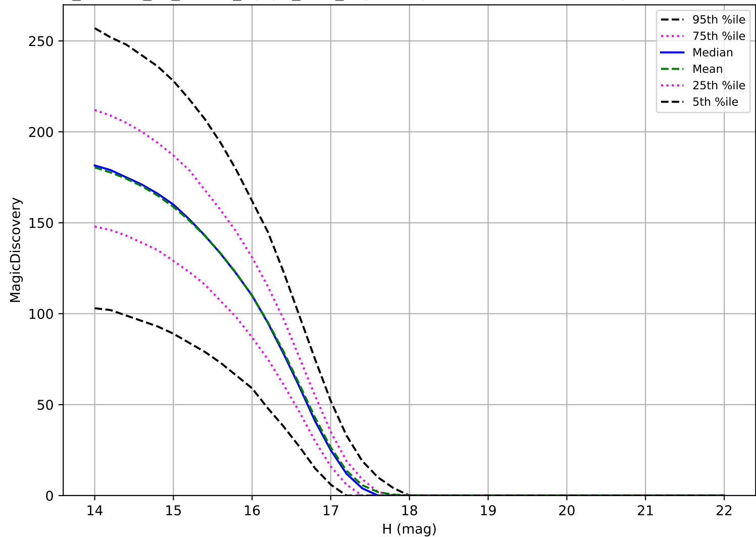
roll_uniform_eh_acc1.0_mjdp0_v3.4_10yrs: Trojan 6 detections in 60 nights detection loss
