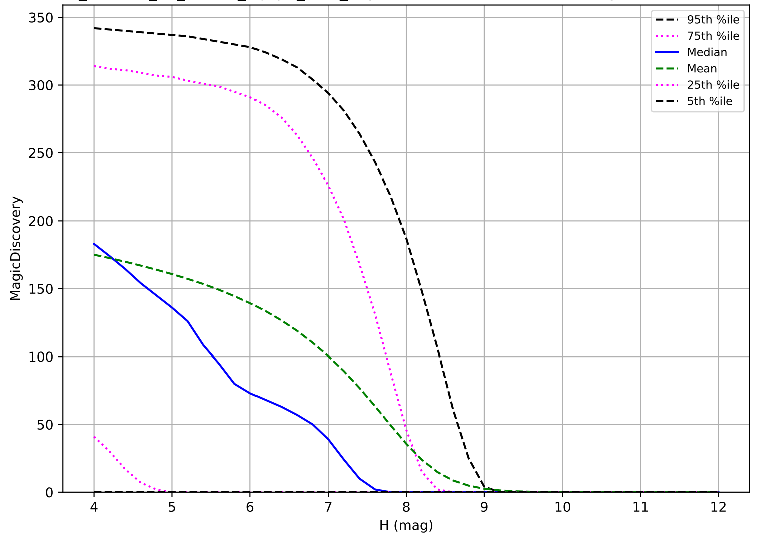
roll_uniform_eh_acc1.0_mjdp0_v3.4_10yrs: TNO 6 detections in 60 nights detection loss
