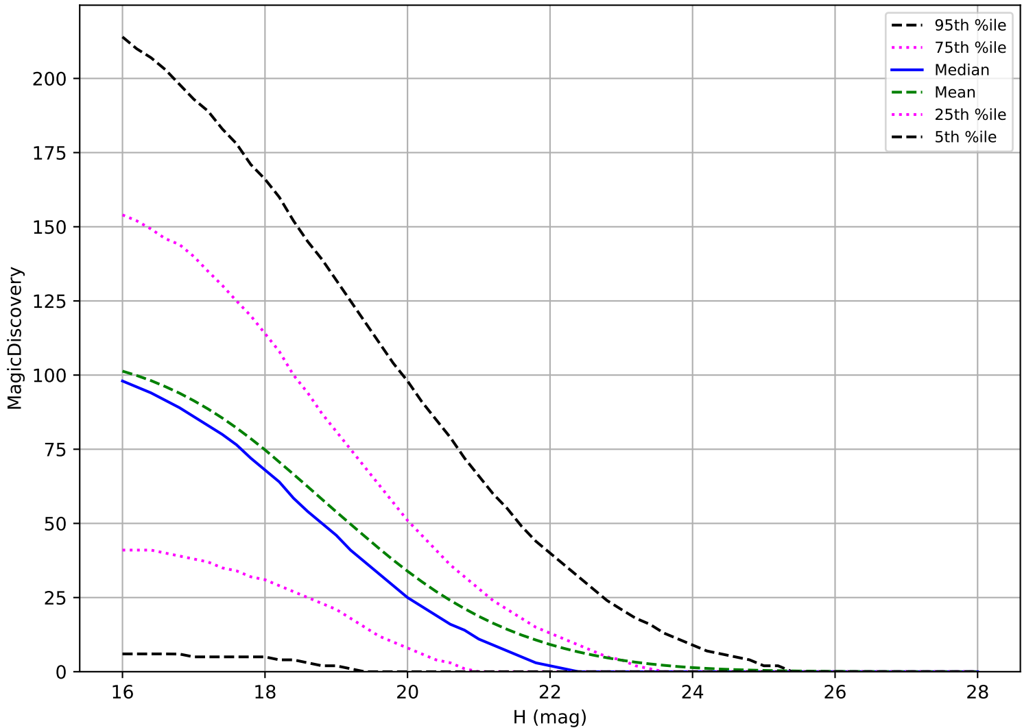
roll_uniform_eh_acc1.0_mjdp0_v3.4_10yrs: PHA 6 detections in 60 nights detection loss
