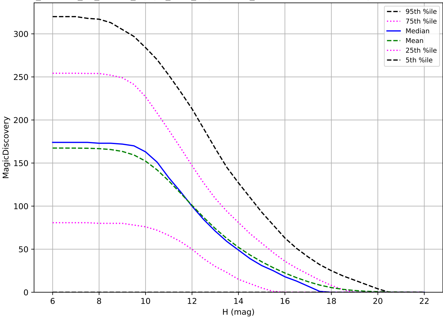
roll_uniform_eh_acc1.0_mjdp0_v3.4_10yrs: OCC_r5 6 detections in 60 nights detection loss
