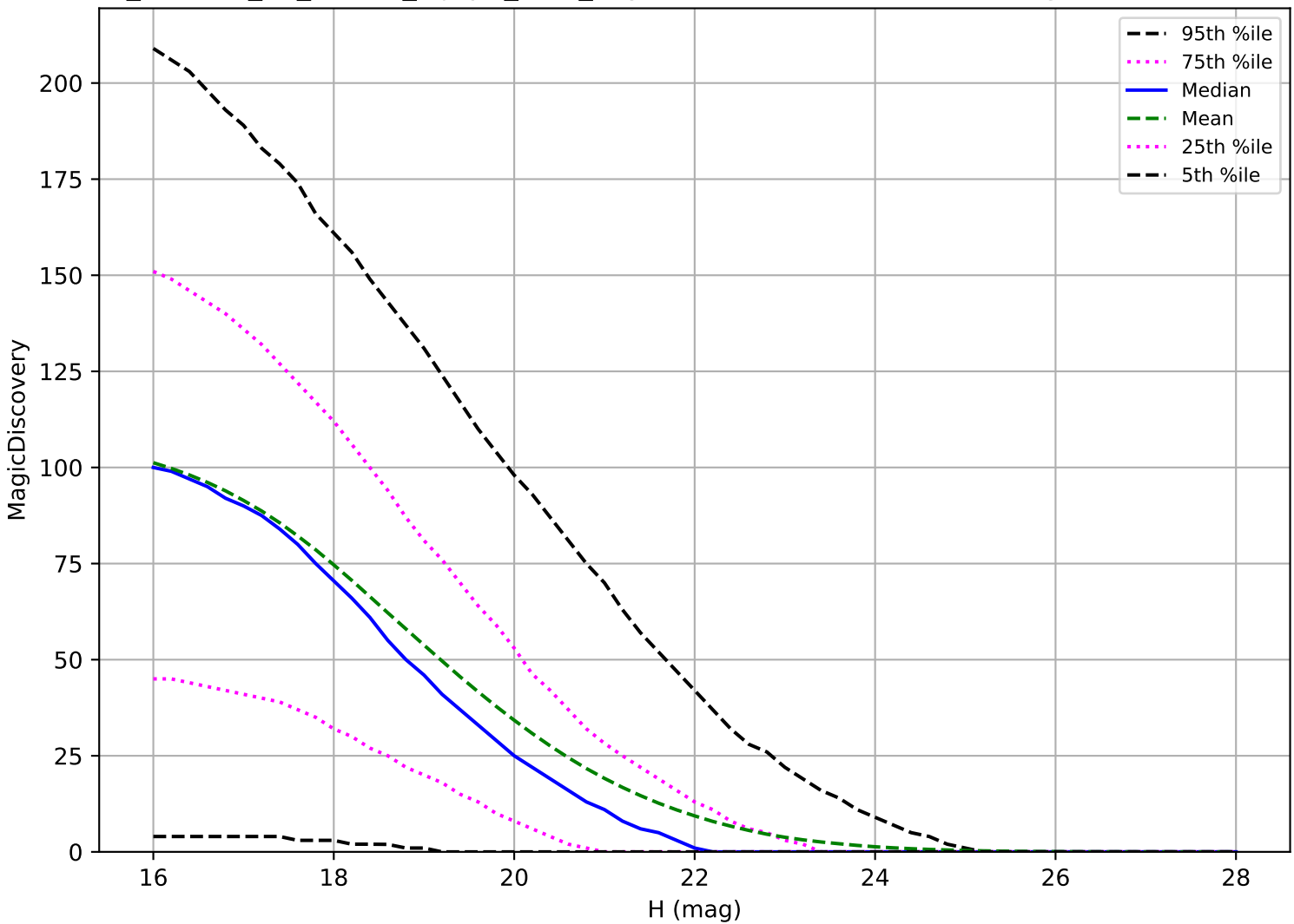
roll_uniform_eh_acc1.0_mjdp0_v3.4_10yrs: NEO 6 detections in 60 nights detection loss
