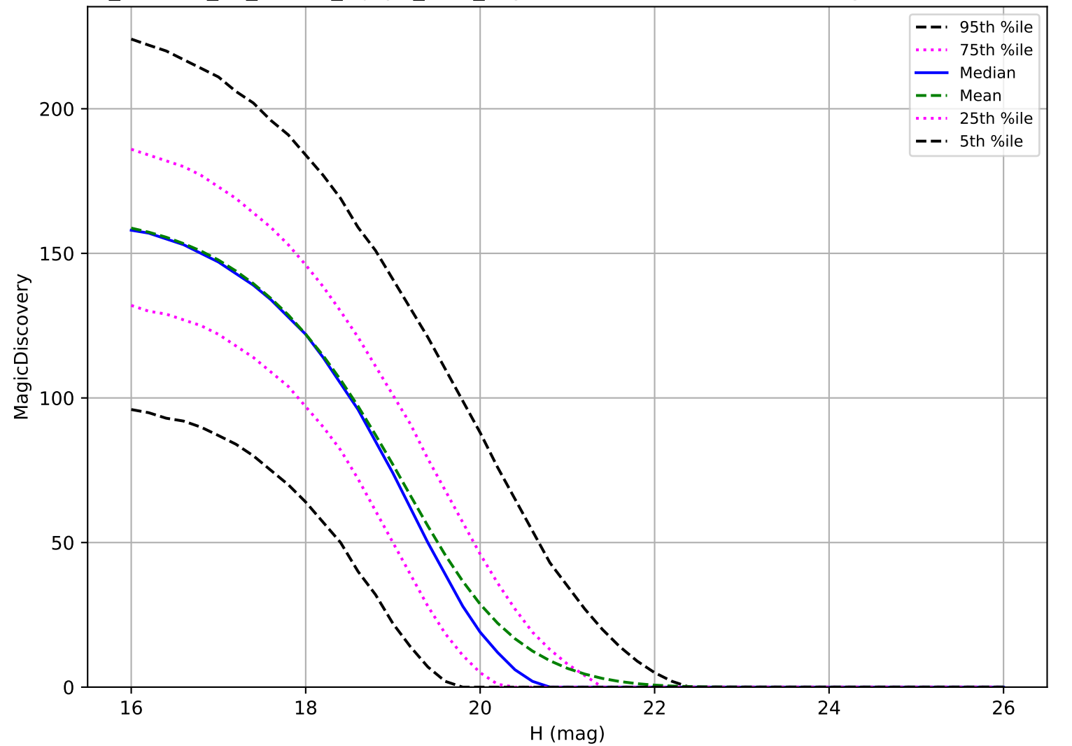
roll_uniform_eh_acc1.0_mjdp0_v3.4_10yrs: MBA 6 detections in 60 nights detection loss
