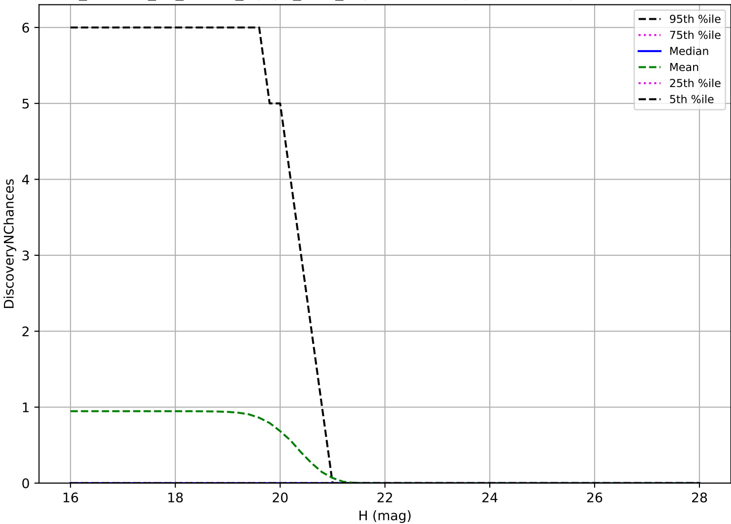
roll_uniform_eh_acc1.0_mjdp0_v3.4_10yrs: Vatira 3 pairs in 15 nights detection loss
