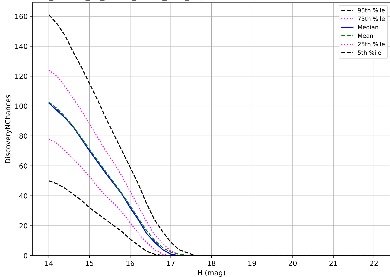
roll_uniform_eh_acc1.0_mjdp0_v3.4_10yrs: Trojan 3 pairs in 15 nights detection loss
