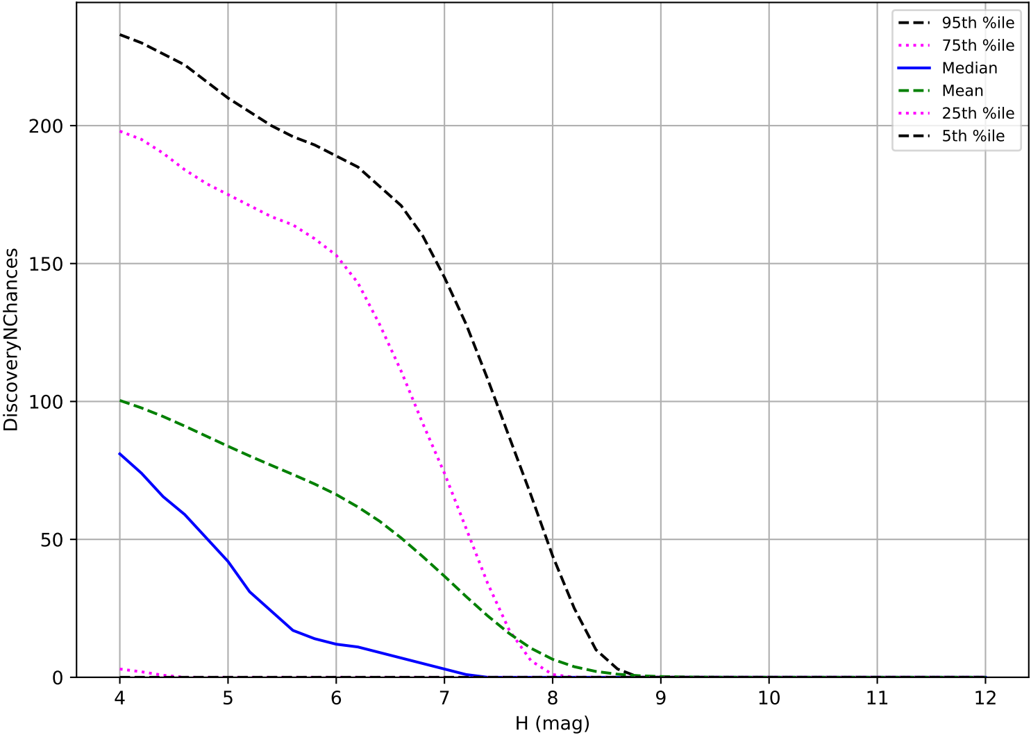
roll_uniform_eh_acc1.0_mjdp0_v3.4_10yrs: TNO 3 pairs in 15 nights detection loss
