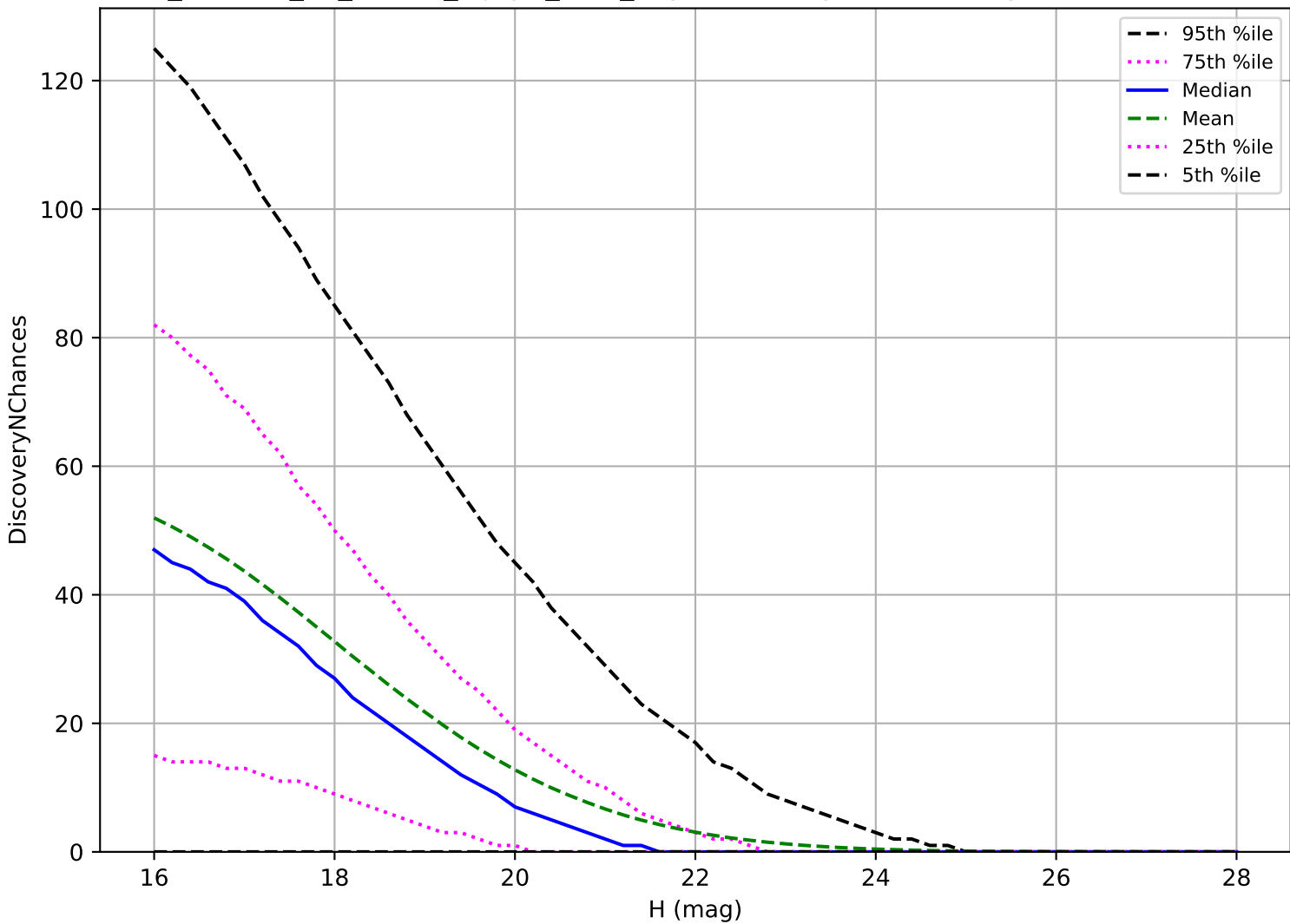
roll_uniform_eh_acc1.0_mjdp0_v3.4_10yrs: PHA 3 pairs in 15 nights detection loss
