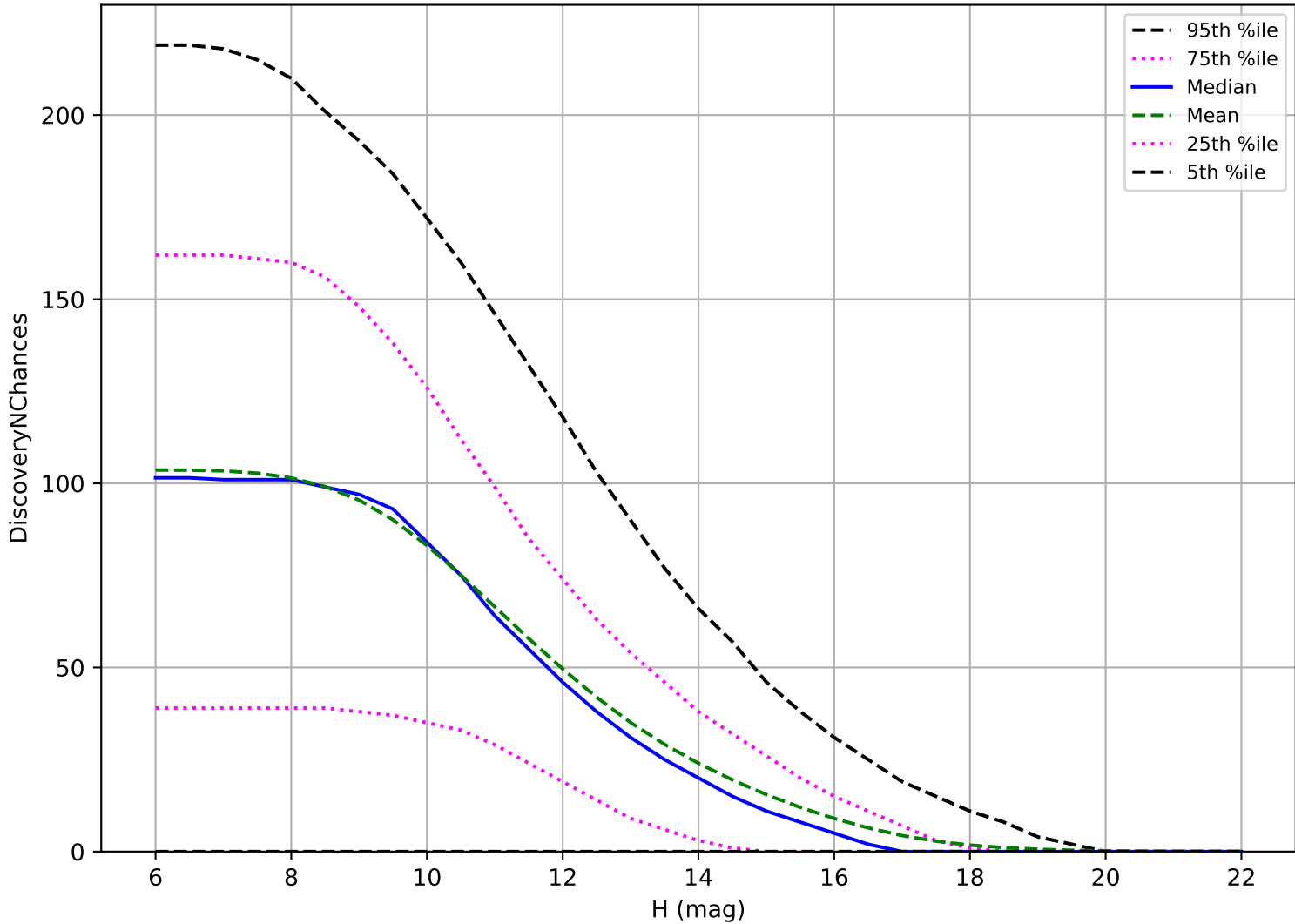
roll_uniform_eh_acc1.0_mjdp0_v3.4_10yrs: OCC_r5 3 pairs in 15 nights detection loss
