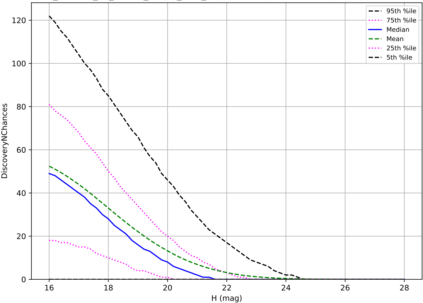
roll_uniform_eh_acc1.0_mjdp0_v3.4_10yrs: NEO 3 pairs in 15 nights detection loss
