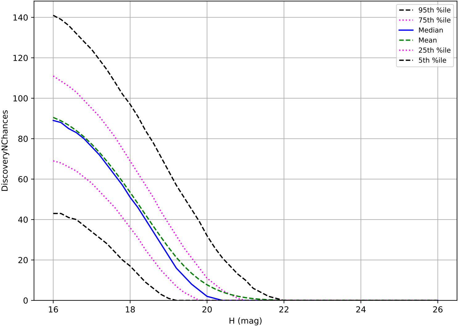
roll_uniform_eh_acc1.0_mjdp0_v3.4_10yrs: MBA 3 pairs in 15 nights detection loss
