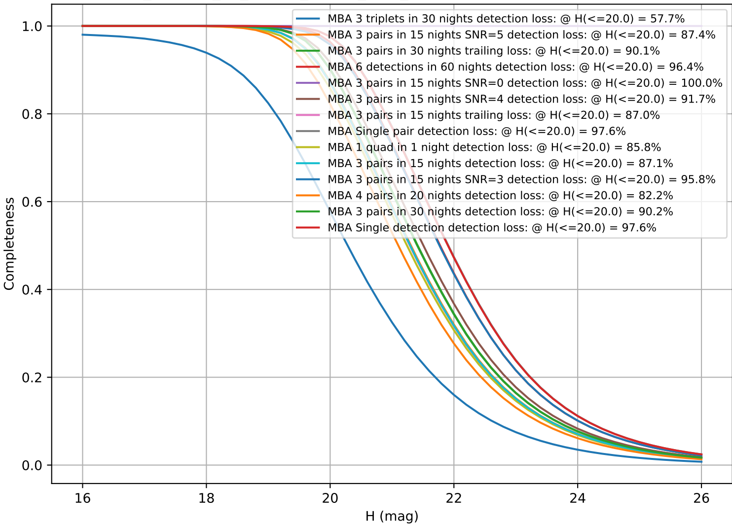
roll_uniform_eh_acc1.0_mjdp0_v3.4_10yrs: CumulativeCompleteness
