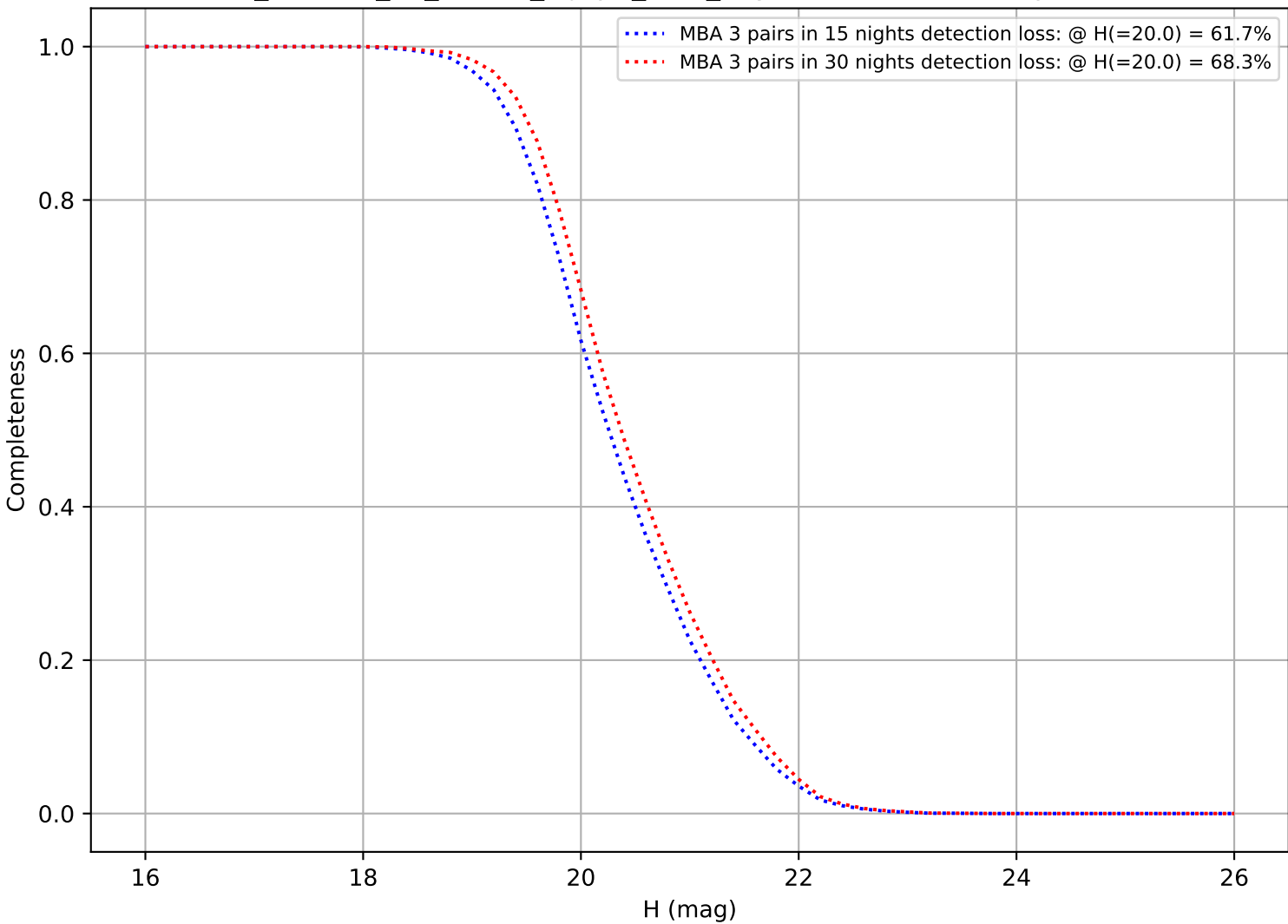
roll_uniform_eh_acc1.0_mjdp0_v3.4_10yrs: DifferentialCompleteness
