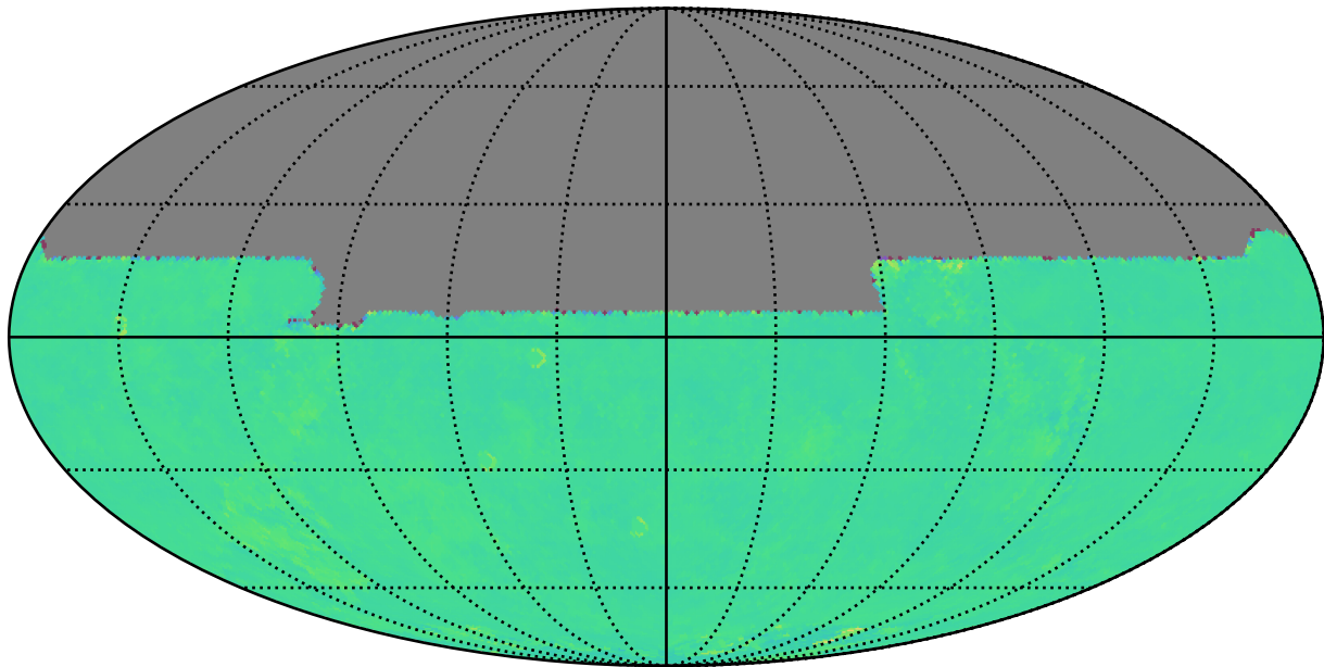
roll_uniform_eh_acc1.0_mjdp0_v3.4_10yrs y: Kuiper rotTelPos
