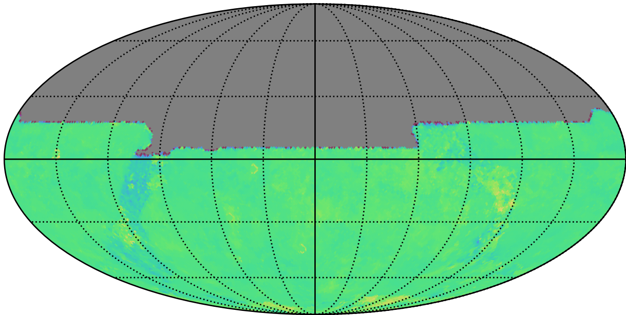
roll_uniform_eh_acc1.0_mjdp0_v3.4_10yrs u: Kuiper rotTelPos
