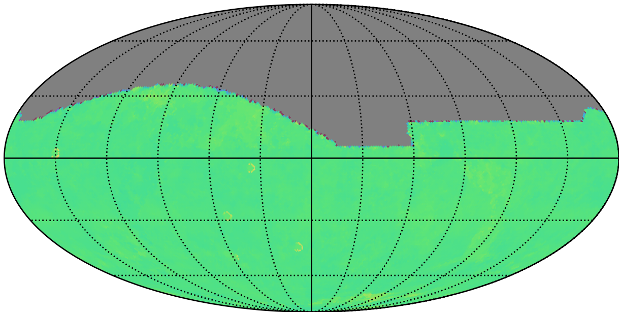
roll_uniform_eh_acc1.0_mjdp0_v3.4_10yrs r: Kuiper rotTelPos
