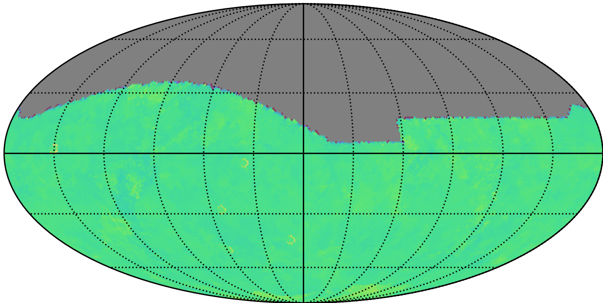
roll_uniform_eh_acc1.0_mjdp0_v3.4_10yrs g: Kuiper rotTelPos
